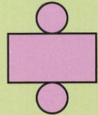
Cylinder
