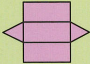
Triangular Prism
