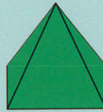
Square-based Pyramid
