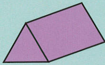
Triangular Prism
