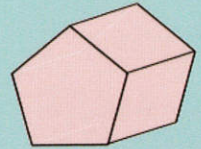
Pentagonal Prism
