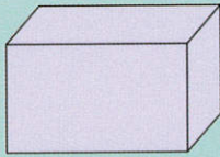
Cuboid
